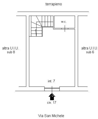
PIANO TERRA Hm= 3,50mt.
